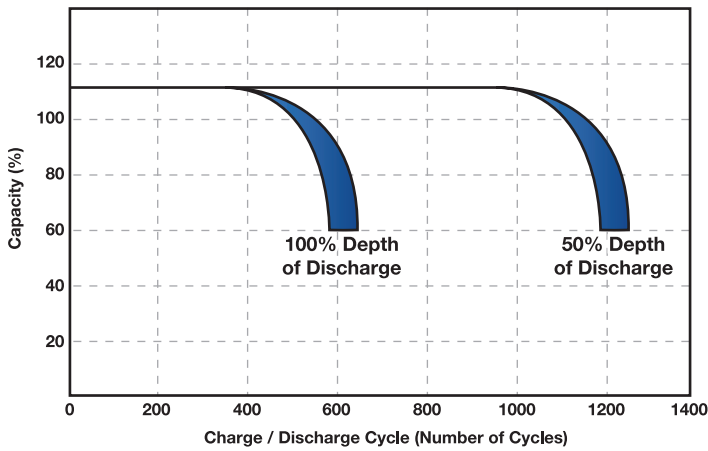
Cycle Life versus Depth of Discharge
