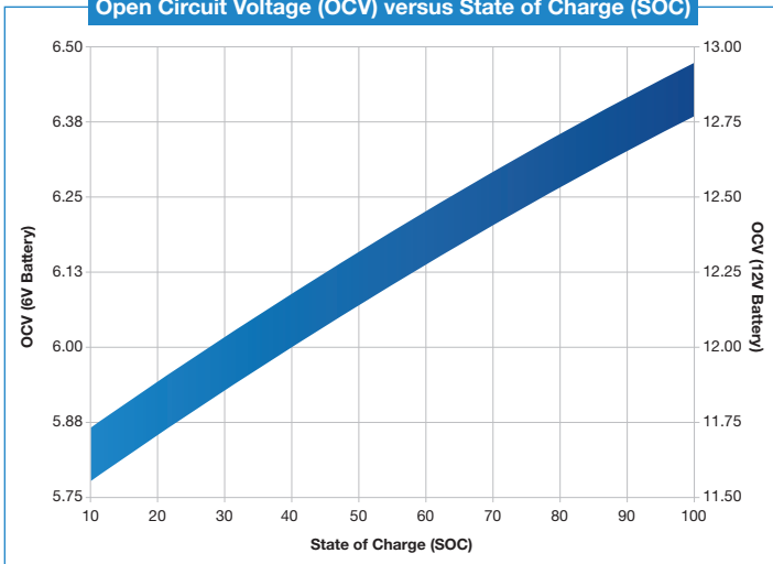
Open Circuit Voltage (OCV) versus State of Charge (SOC)
