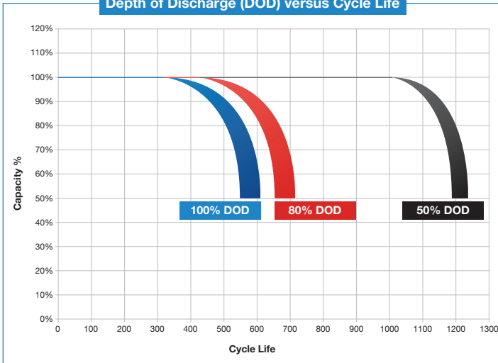
Depth of Discharge (DOD) versus Cycle Life
