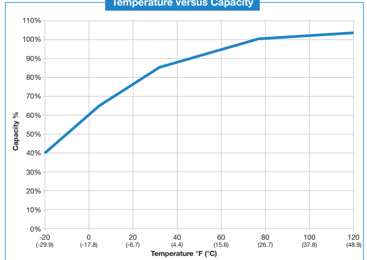
Temperature versus Capacity
