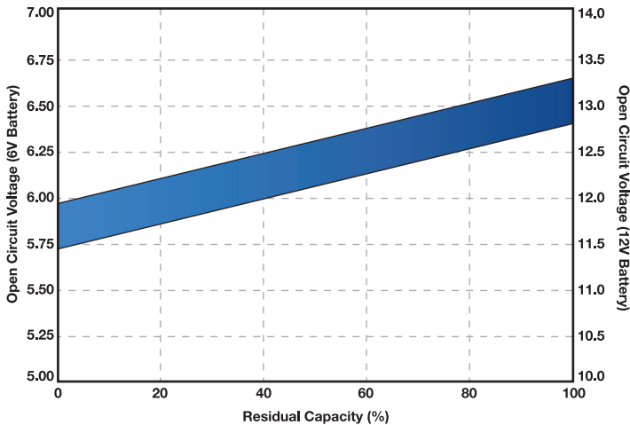
Open Circuit Voltage versus State of Charge
